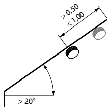
Fig. 12 Rooms with slanted ceilings
